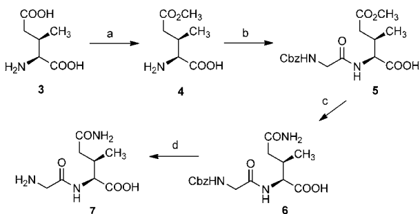
Scheme 2. Synthesis of Gly-mGln: a) \text{SOCl}_2 , MeOH; 30 min at -20^\circ\text{C} to 5^\circ\text{C} under \text{N}_2 (91 %); b) Cbz-Gly-OSu, \text{NaHCO}_3 (10%) aqueous solution, 1,4-dioxane; 30 min at RT (78 %); c) 28 % aqueous \text{NH}_4\text{OH} ; 18 h at RT (65 %); d) \text{H}_2 /10 % Pd/C in MeOH.
